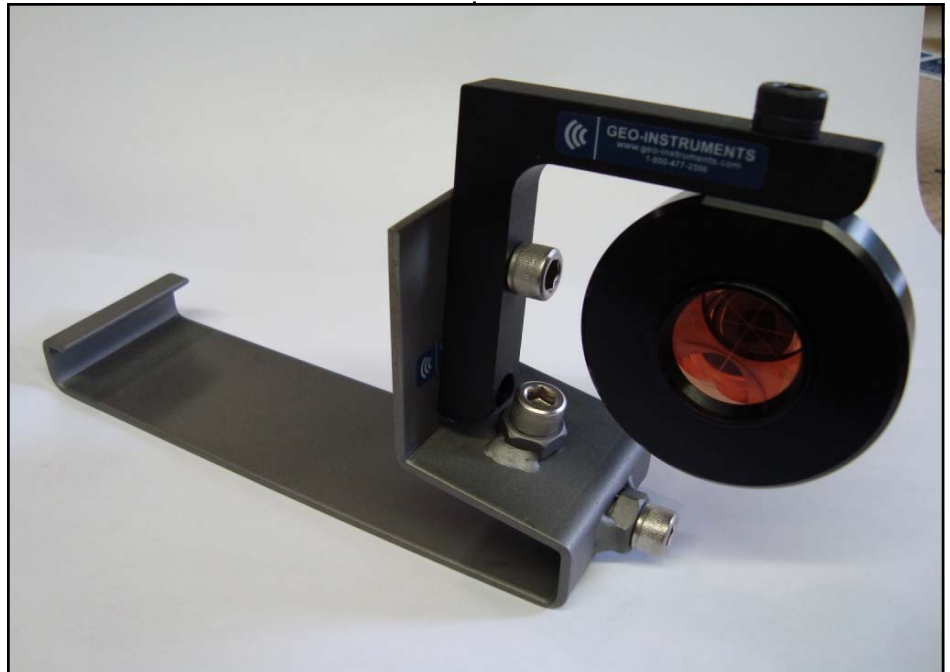
Above: Track Clip and Geo-Instruments 25.4 mini prism
